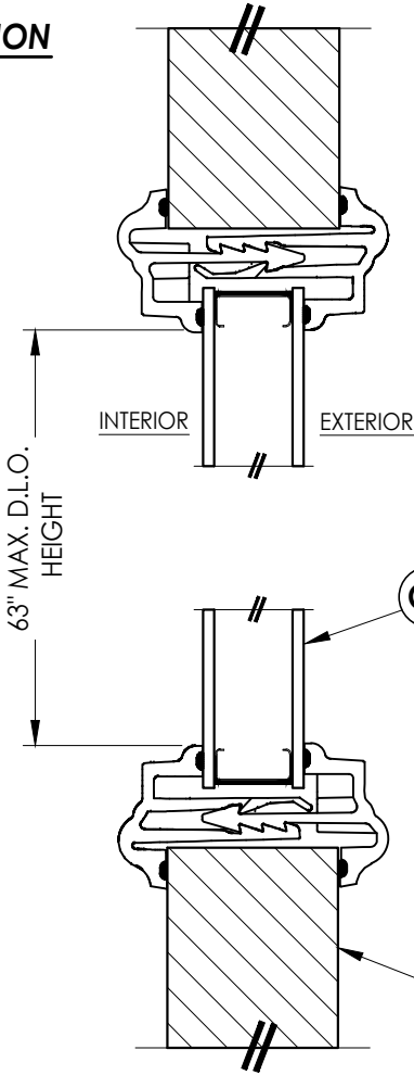
1 2 VERTICAL CROSS SECTION
